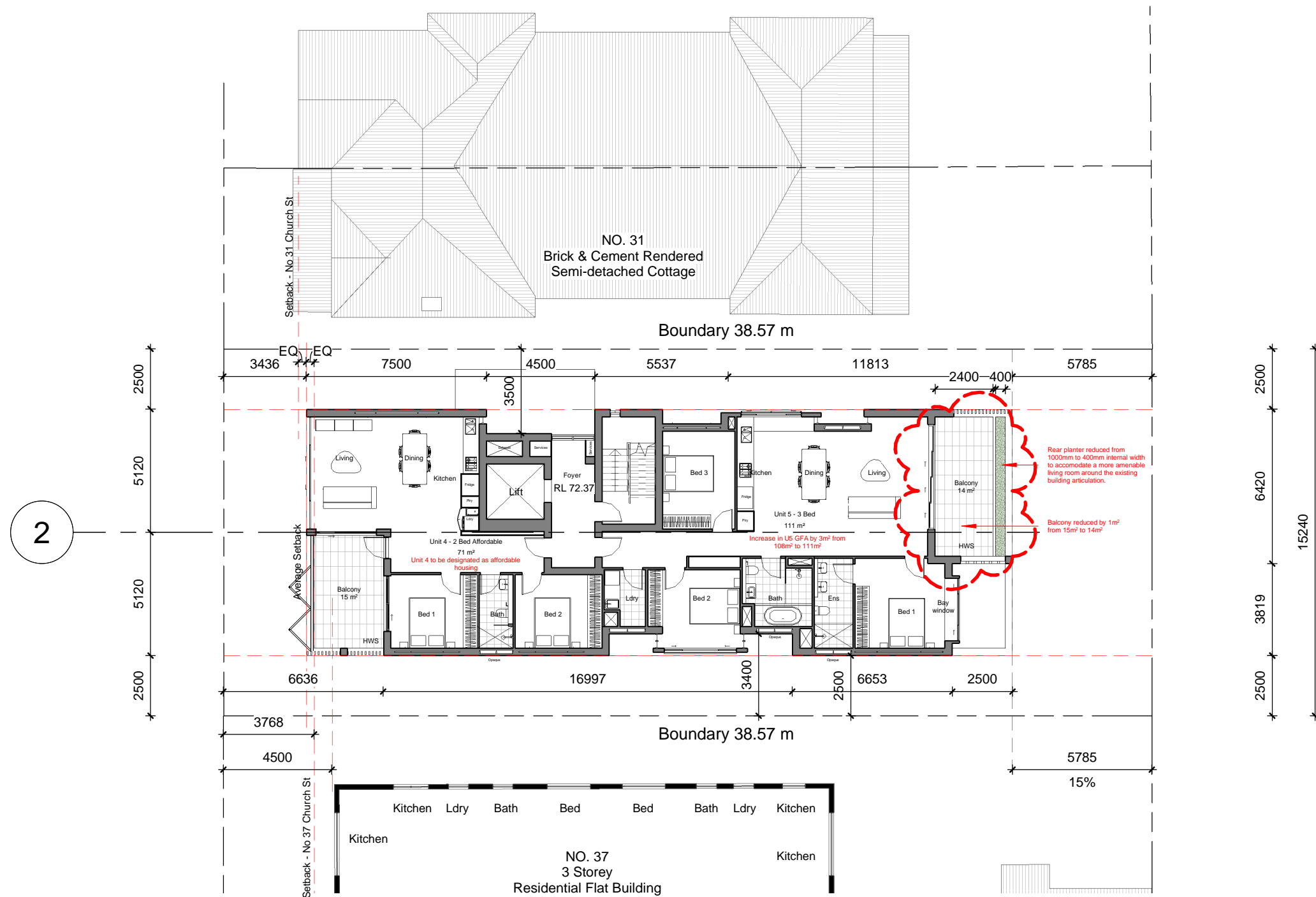
1. Level 1 Scale 1 : 200
